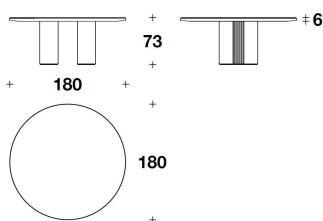
TTV (39E) - TTV (39M) TAVOLO / TABLE Ø 180x73H. - THK.6cm Ø 71x28 2/3H. - THK.2 6/16"
