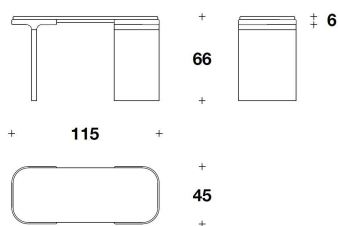
COT (03/2) LOW : CONSOLLE / CONSOLE 115x45x66H.cm 45 1/3x17 3/4x26H."
