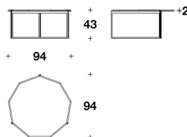
LYC (42) MEDIUM : SIDE TABLE 94x94x43H. cm 37x37x17H. "
