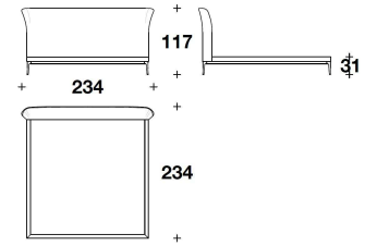
HEE (LE7) LETTO PER MATERASSO / BED FOR MATTRESS 200x200 - 234x234x117H. - H.B.31cm 78 2/3x78 2/3 - 92x92x46H. - H.B.12 1/4"
