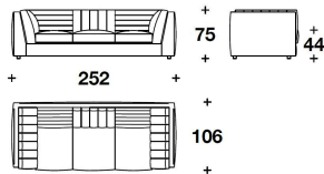
IAA (D3) DIVANO 3 POSTI / 3 SEATER SOFA 252x106x75H. - H.S.44cm 99 1/3x41 2/3x29 2/3H. - H.S.17 1/4"
