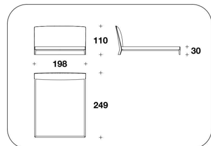
NWE (CUSA) CALIFORNIA USA : LETTO PER MATERASSO / BED FOR MATTRESS 183x215 - 198x249x110H. - H.B.30cm 72x84 2/3 - 78x98x43 1/3H. - H.B.11 3/4"
