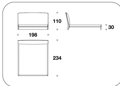
NWE (ELE2) VENEERED : LETTO PER MATERASSO / BED FOR MATTRESS 185x200 - 198x234x110H. - H.B.30cm 73x78 2/3 - 78x92x43 1/3H. - H.B.11 3/4"
