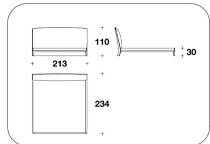
NWE (ELE7) VENEERED : LETTO PER MATERASSO / BED FOR MATTRESS 200x200 - 213x234x110H. - H.B.30cm 78 2/3x78 2/3 - 84x92x43 1/3H. - H.B.11 3/4"
