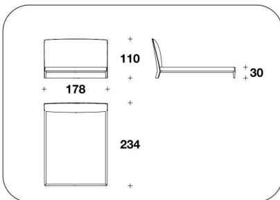
NWE (ELE1) VENEERED : LETTO PER MATERASSO / BED FOR MATTRESS 165x200 - 178x234x110H. - H.B.30cm 65x78 2/3 - 70x92x43 1/3H. - H.B.11 3/4"
