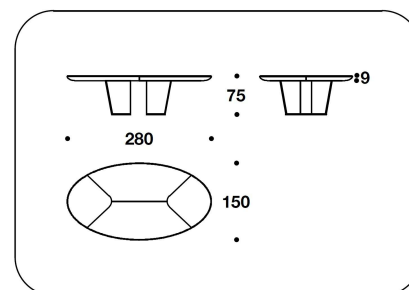
BTV (03P) - BTV (03) TAVOLO OVALE / OVAL TABLE 280x150x75H. - THK.9cm 110 1/3x59x29 2/3H. - THK.3 2/4"
