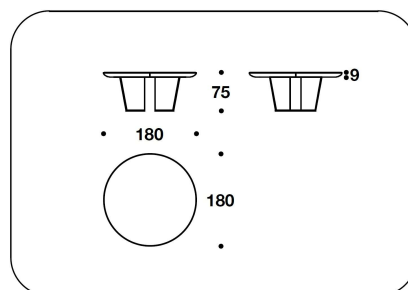
BTV (02P) - BTV (02) TAVOLO TONDO / ROUND TABLE Ø 180x75H. - THK.9cm Ø 71x29 2/3H. - THK.3 2/4"
