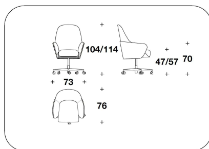
POB (22E) VENEERED : POLTRONA DA UFFICIO / OFFICE ARMCHAIR 73x76x104/114H. - H.S.47/57 cm 28 2/3x30x41/45H. - H.S.18 2/4/22 1/3 "
