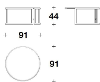
TCV (53E) COFFEE TABLE Ø 91x44H. cm Ø 35 2/3x17 1/4H. "
