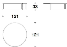
TCV (54E) COFFEE TABLE Ø 121x33H. cm Ø 47 2/3x13H. "
