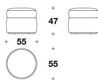
PUP (POUP) - PUP (POUP1) POUF / OTTOMAN Ø 55x47H.cm Ø 21 2/3x18 2/4H."
