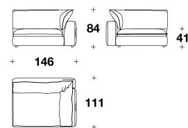
SOT (ED) - SOT (ES) BIG : ELEMENTO CON BRACCIOLO DX O SX / ELEMENT WITH RIGHT OR LEFT ARMREST 146x111x84H. - HS.41cm 57 1/3x43 2/3x33H. - HS.16 1/4"
