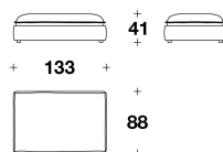
SOT (POUR) POUF RETTANGOLARE / RECTANGULAR OTTOMAN 133x88x41H.cm 52 1/3x34 2/3x16 1/4H."
