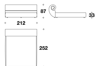
RIC (LE7) LETTO PER MATERASSO / BED FOR MATTRESS 200x200 - 212x252x87H. - H.B.33cm 78 2/3x78 2/3 - 83 1/3x99 1/3x34 1/3H. - H.B.13"
