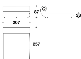
RIC (KUSA) KING USA : LETTO PER MATERASSO / BED FOR MATTRESS 195x205 - 207x257x87H. - H.B.33cm 76 2/3x80 2/3 - 81 1/3x101 1/3x34 1/3H. - H.B.13"
