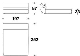
RIC (LE2) LETTO PER MATERASSO / BED FOR MATTRESS 185x200 - 197x252x87H. - H.B.33cm 73x78 2/3 - 77 2/3x99 1/3x34 1/3H. - H.B.13"
