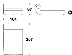
RIC (QUSA) QUEEN USA : LETTO PER MATERASSO / BED FOR MATTRESS 152x205 - 164x257x87H. - H.B.33cm 60x80 2/3 - 64 2/3x101 1/3x34 1/3H. - H.B.13"
