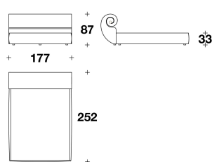
RIC (LE1) LETTO PER MATERASSO / BED FOR MATTRESS 165x200 - 177x252x87H. H.B.33cm 65x78 2/3 - 69 2/3x99 1/3x34 1/3H. H.B.13"
