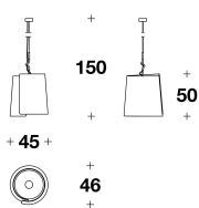
TRL (38) SMALL : SOSPENSIONE / SUSPENSION 45x46x150H.cm 17 3/4x18x59H."
