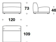
1BL (ECG) BIG : ELEMENTO CENTRALE 1 POSTO / 1 SEATER CENTRAL ELEMENT 120x109x73H. - H.S.46cm 47 1/3x43x28 2/3H. - H.S.18"
