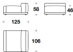
1BL (POUG) POUF QUADRATO CON BRACCIOLO / SQUARE OTTOMAN WITH ARMREST 125x106x58H. - H.S.46cm 49 1/3x41 2/3x23H. - H.S.18"
