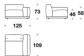
1BL (EDP) - 1BL (ESP) ELEMENTO 1 POSTO CON BRACCIOLO DX O SX / 1 SEATER ELEMENT WITH RIGHT OR LEFT ARMREST 125x109x73H. - H.S.46cm 49 1/3x43x28 2/3H. - H.S.18"
