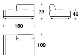
1BL (PEND) - 1BL (PENS) ELEMENTO PENISOLA 1 POSTO CON POUF DX O SX / 1 SEATER PENINSULA ELEMENT WITH RIGHT OR LEFT OTTOMAN 160x109x73H. - H.S.46cm 63x43x28 2/3H. - H.S.18"
