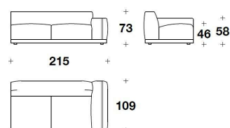
1BL (E3D) - 1BL (E3S) ELEMENTO 3 POSTI CON BRACCIOLO DX O SX / 3 SEATER ELEMENT WITH RIGHT OR LEFT ARMREST 215x109x73H. - H.S.46cm 84 2/3x43x28 2/3H. - H.S.18"
