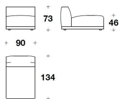
1BL (ECPC) COMFORT : ELEMENTO CENTRALE 1 POSTO / 1 SEATER CENTRAL ELEMENT 90x134x73H. - H.S.46cm 35 1/3x52 2/3x28 2/3H. - H.S.18"
