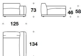
1BL (EDPC) - 1BL (ESPC) COMFORT : ELEMENTO 1 POSTO CON BRACCIOLO DX O SX / 1 SEATER ELEMENT WITH RIGHT OR LEFT ARMREST 125x134x73H. - H.S.46cm 49 1/3x52 2/3x28 2/3H. - H.S.18"
