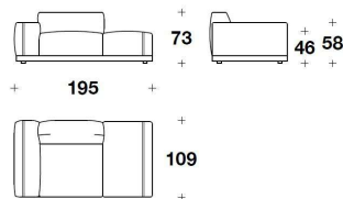
1BL (PENDT) - 1BL (PENST) ELEMENTO PENISOLA 1 POSTO CON BRACCIOLO DX O SX E POUF / 1 SEATER PENINSULA ELEMENT WITH RIGHT OR LEFT ARMREST AND OTTOMAN 195x109x73H. - H.S.46cm 76 2/3x43x28 2/3H. - H.S.18"
