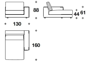
SQU (CLD) - SQU (CLS) CHAISE LONGUE 1 POSTO CON BRACCIOLO DX O SX / 1 SEATER CHAISE LONGUE WITH RIGHT OR LEFT ARMREST 130x160x88H. – H.S.44cm 51 1/3x63x34 2/3H. – H.S.17 1/4"
