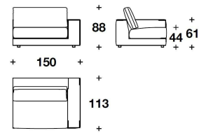
SQU (E1D) - SQU (E1S) BIG : ELEMENTO 1 POSTO CON BRACCIOLO DX O SX / 1 SEATER ELEMENT WITH RIGHT OR LEFT ARMREST 150x113x88H. – H.S.44cm 59x44 1/3x34 2/3H. – H.S.17 1/4"
