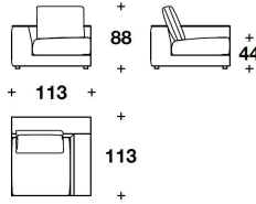
SQU (ANG) ELEMENTO ANGOLARE QUADRATO / SQUARE CORNER ELEMENT 113x113x88H. – H.S.44cm 44 1/3x44 1/3x34 2/3H. – H.S.17 1/4"
