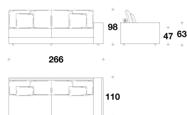
ELN (AE4AD) - ELN (AE4AS) ELEMENTO ANGOLARE 4 POSTI CON ANGOLO DX O SX / 4 SEATER CORNER ELEMENT WITH RIGHT OR LEFT CORNER 266x110x98H. - H.S.47cm 104 2/3x43 1/3x38 2/3H. - H.S.18 2/4"
