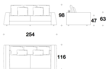
ELN (AD2) DIVANO 2 POSTI / 2 SEATER SOFA 254x116x98H. - H.S.47cm 100x45 2/3x38 2/3H. - H.S.18 2/4"
