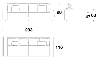
ELN (AD4AD) - ELN (AD4AS) DIVANO ANGOLARE 4 POSTI CON BRACCIOLO DX O SX / 4 SEATER CORNER SOFA WITH RIGHT OR LEFT ARMREST 293x116x98H. - H.S.47cm 115 1/3x45 2/3x38 2/3H. - H.S.18 2/4"
