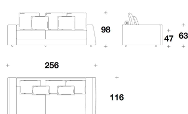
ELN (AD1AD) - ELN (AD1AS) DIVANO ANGOLARE 1 POSTO CON BRACCIOLO DX O SX / 1 SEATER CORNER SOFA WITH RIGHT OR LEFT ARMREST 256x116x98H. - H.S.47cm 100 2/3x45 2/3x38 2/3H. - H.S.18 2/4"
