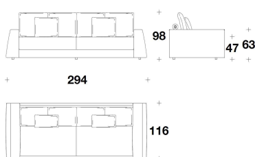
ELN (AD4) DIVANO 4 POSTI / 4 SEATER SOFA 294x116x98H. - H.S.47cm 115 2/3x45 2/3x38 2/3H. - H.S.18 2/4"
