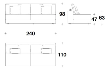
ELN (AE4C) ELEMENTO CENTRALE 4 POSTI / 4 SEATER CENTRAL ELEMENT 240x110x98H. - H.S.47cm 94 1/3x43 1/3x38 2/3H. - H.S.18 2/4"
