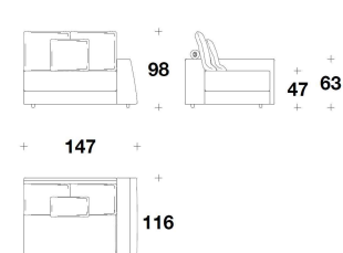
ELN (AE1D) - ELN (AE1S) ELEMENTO 1 POSTO CON BRACCIOLO DX O SX / 1 SEATER ELEMENT WITH RIGHT OR LEFT ARMREST 147x116x98H. - H.S.47cm 58x45 2/3x38 2/3H. - H.S.18 2/4"
