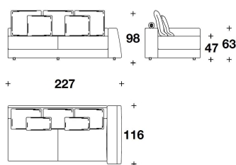
ELN (AE2D) - ELN (AE2S) ELEMENTO 2 POSTI CON BRACCIOLO DX O SX / 2 SEATER ELEMENT WITH RIGHT OR LEFT ARMREST 227x116x98H. - H.S.47cm 89 1/3x45 2/3x38 2/3H. - H.S.18 2/4"
