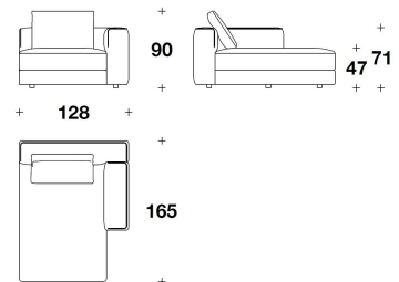
GON (CLD) - GON (CLS) CHAISE LONGUE 1 POSTO CON BRACCIOLO DX O SX / 1 SEATER CHAISE LONGUE WITH RIGHT OR LEFT ARMREST 128x165x90H. – H.S.47cm 50 1/3x65x35 1/3H. – H.S.18 2/4"
