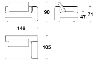
GON (EDG) - GON (ESG) BIG : ELEMENTO 1 POSTO CON BRACCIOLO DX O SX / 1 SEATER ELEMENT WITH RIGHT OR LEFT ARMREST 148x105x90H. – H.S.47cm 58 1/3x41 1/3x35 1/3H. – H.S.18 2/4"
