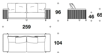
1CO (D3) DIVANO 3 POSTI / 3 SEATER SOFA 259x104x96H. – H.S.46cm 102x41x37 2/3H. – H.S.18"
