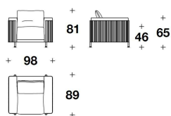
1CO (POL) POLTRONA / ARMCHAIR 98x89x81H. – H.S.46cm 38 2/3x35x32H. – H.S.18"
