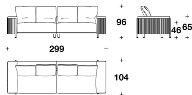
1CO (D4) DIVANO 4 POSTI IN 2 ELEMENTI / 4 SEATER SOFA IN 2 ELEMENTS 299x104x96H. – H.S.46cm 117 2/3x41x37 2/3H. – H.S.18"
