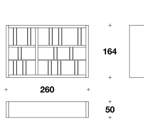
MBT (25B) LIBRERIA BASSA / LOW BOOKSHELF 260x50x164H.cm 102 1/3x19 3/4x64 2/3H."
