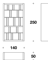
MBT (25A) LIBRERIA ALTA / HIGH BOOKSHELF 140x50x250H.cm 55x19 3/4x98 1/3H."
