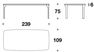
TTV (21MF) TAVOLO RETTANGOLARE / RECTANGULAR TABLE 239x109x75H. - THK.6 cm 94x43x29 2/3H. - THK.2 6/16 "
