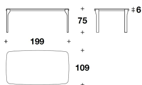
TTV (20MF) TAVOLO RETTANGOLARE / RECTANGULAR TABLE 199x109x75H. - THK.6 cm 78 1/3x43x29 2/3H. - THK.2 6/16 "
