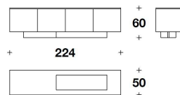
MBT (30E) - 1TV (05) LOW CABINET 224x50x60H. cm 88 1/3x19 3/4x23 2/3H. "
