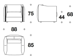
DLS (POL) POLTRONA / ARMCHAIR 88x85x75H. - H.S.44cm 34 2/3x33 1/3x29 2/3H. - H.S.17 1/4"
