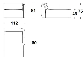
DLS (CLD) - DLS (CLS) CHAISE LONGUE 1 POSTO CON BRACCIOLO DX O SX / 1 SEATER CHAISE LONGUE WITH RIGHT OR LEFT ARMREST 112x160x81H. - H.S.46cm 44x63x32H. - H.S.18"
