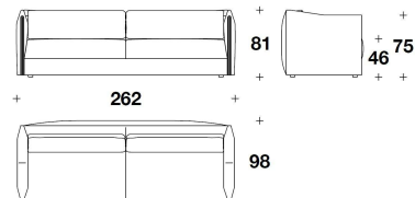
DLS (D4) DIVANO 4 POSTI / 4 SEATER SOFA 262x98x81H. - H.S.46cm 103x38 2/3x32H. - H.S.18"
