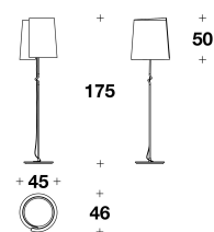
TRL (36) LAMPADA DA TERRA / FLOOR LAMP 45x46x175H.cm 17 3/4x18x69H."
