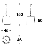
TRL (38) SMALL : SOSPENSIONE / SUSPENSION 45x46x150H.cm 17 3/4x18x59H."
