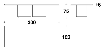
DTV (19L) - DTV (19R) TAVOLO RETTANGOLARE / RECTANGULAR TABLE 300x120x75H. - THK.6cm 118x47 1/3x29 2/3H. - THK.2 6/16"
