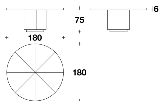
DTV (21L) - DTV (21R) TAVOLO TONDO / ROUND TABLE Ø 180x75H. - THK.6 cm Ø 71x29 2/3H. - THK.2 6/16 "
