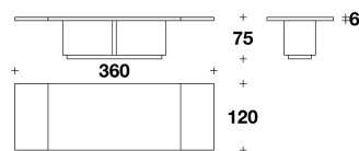
DTV (18L) - DTV (18R) TAVOLO RETTANGOLARE / RECTANGULAR TABLE 360x120x75H. - THK.6cm 141 1/2x47 1/3x29 2/3H. - THK.2 6/16"
