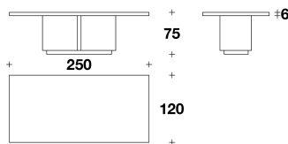
DTV (20L) - DTV (20R) TAVOLO RETTANGOLARE / RECTANGULAR TABLE 250x120x75H. - THK.6cm 98 1/3x47 1/3x29 2/3H. - THK.2 6/16"
