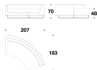
GHA (ECD) - GHA (ECS) ELEMENTO CURVO DX O SX / RIGHT OR LEFT CURVED ELEMENT 207x183x70H. - H.S.48cm 81 1/3x72x27 2/3H. - H.S.19"
