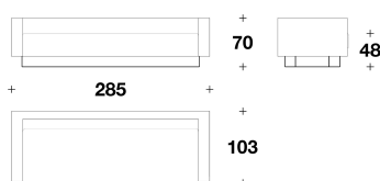
GHA (D4) DIVANO 4 POSTI / 4 SEATER SOFA 285x103x70H. - H.S.48cm 112 1/3x40 2/3x27 2/3H. - H.S.19"
