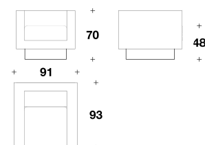
GHA (POL) POLTRONA / ARMCHAIR 91x93x70H. - H.S.48cm 35 2/3x36 2/3x27 2/3H. - H.S.19"
