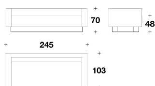
GHA (D3) DIVANO 3 POSTI / 3 SEATER SOFA 245x103x70H. - H.S.48cm 96 1/3x40 2/3x27 2/3H. - H.S.19"
