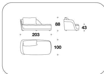
RCM (CLD) - RCM (CLS) CHAISE LONGUE DX O SX / RIGHT OR LEFT CHAISE LONGUE 203x100x88H. - H.S.43cm 80x39 1/3x34 2/3H. - H.S.17"
