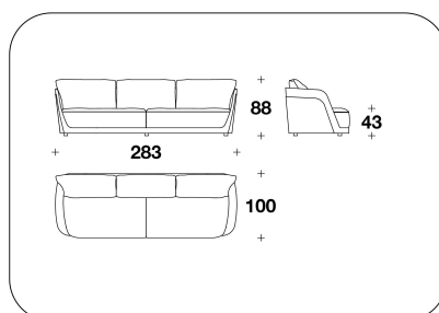
RCM (D3ME) - RCM (D3ME/SCZ) MAXI : DIVANO 3 POSTI / 3 SEATER SOFA 283x100x88H. - H.S.43cm 111 1/3x39 1/3x34 2/3H. - H.S.17"
