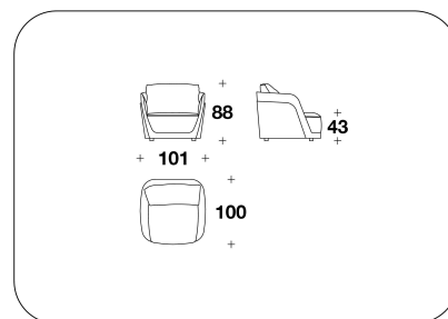
RCM (POLE) - RCM (POLE/SCZ) POLTRONA / ARMCHAIR 101x100x88H. - H.S.43cm 39 2/3x39 1/3x34 2/3H. - H.S.17"
