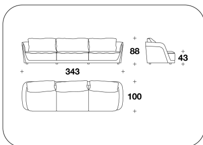
RCM (D4) DIVANO 4 POSTI / 4 SEATER SOFA 343x100x88H. - H.S.43cm 135x39 1/3x34 2/3H. - H.S.17"
