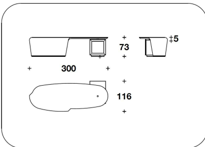
BTV (18MP) - BTV (18ME) - BTV (18CP) - BTV (18CE) OPTIONAL 1 - OPTIONAL 2 x BTV (18) L.300x116x73H. - 307x246x73H.cm L.118x45 2/3x28 2/3H. - 121x97x28 2/3H."
