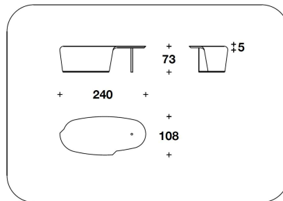
BTV (19PE) TOP SYCAMORE - BURR WALNUT : SCRIVANIA DX O SX / RIGHT OR LEFT WRITING-DESK L.240x108x73H. - 247x246x73H.cm L.94 1/3x42 2/3x28 2/3H. - 97 1/3x97x28 2/3H."
