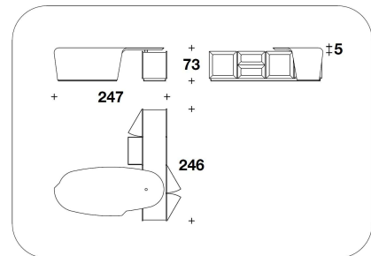
BTV (19PEMP) - BTV (19PEME) - BTV (19PECP) - BTV (19PECE) OPTIONAL 1 - OPTIONAL 2 x BTV (19PE) L.240x108x73H. - 247x246x73H.cm L.94 1/3x42 2/3x28 2/3H. - 97 1/3x97x28 2/3H."
