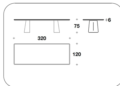
BTV (42M) RECTANGULAR MARBLE : TAVOLO / TABLE 320x120x75H. - THK.6cm 126x47 1/3x29 2/3H. - THK.2 6/16"
