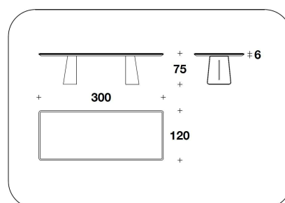
BTV (41M) RECTANGULAR MARBLE : TAVOLO / TABLE 300x120x75H. - THK.6cm 118x47 1/3x29 2/3H. - THK.2 6/16"
