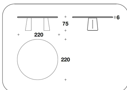
BTV (39E) - BTV (39E/SCZ) MATT VENEERED : TAVOLO TONDO / ROUND TABLE Ø 220x75H. - THK.6cm Ø 86 2/3x29 2/3H. - THK.2 6/16"
