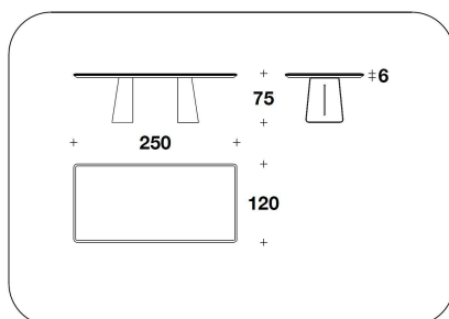
BTV (40E) - BTV (40E/SCZ) MATT VENEERED : TAVOLO RETTANGOLARE / RECTANGULAR TABLE 250x120x75H. - THK.6cm 98 1/3x47 1/3x29 2/3H. - THK.2 6/16"
