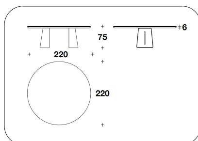
BTV (39E) - BTV (39E/SCZ) GLOSSY VENEERED : TAVOLO TONDO / ROUND TABLE Ø 220x75H. - THK.6 cm Ø 86 2/3x29 2/3H. - THK.2 6/16 "
