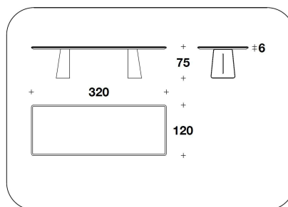
BTV (42E) - BTV (42E/SCZ) GLOSSY VENEERED : TAVOLO RETTANGOLARE / RECTANGULAR TABLE 320x120x75H. - THK.6 cm 126x47 1/3x29 2/3H. - THK.2 6/16 "
