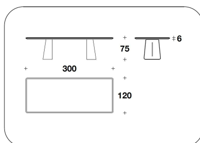
BTV (41E) - BTV (41E/SCZ) GLOSSY VENEERED : TAVOLO RETTANGOLARE / RECTANGULAR TABLE 300x120x75H. - THK.6 cm 118x47 1/3x29 2/3H. - THK.2 6/16 "
