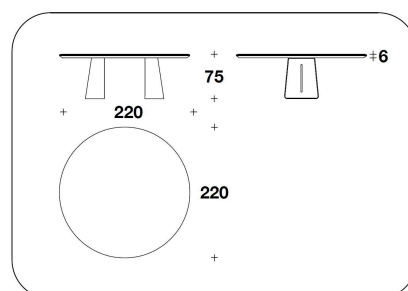
BTV (39M) ROUND MARBLE : TAVOLO / TABLE Ø 220x75H. - THK.6cm Ø 86 2/3x29 2/3H. - THK.2 6/16"
