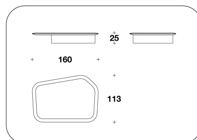
CTB (44E) MATT VENEERED TOP : COFFEE TABLE 160x113x25H.cm 63x44 1/3x9 3/4H."
