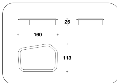
CTB (44EM) GLOSSY VENEERED TOP+TOP INSERT : COFFEE TABLE 160x113x25H.cm 63x44 1/3x9 3/4H."
