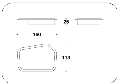
CTB (44M) NATURAL STONE TOP : COFFEE TABLE 160x113x25H.cm 63x44 1/3x9 3/4H."
