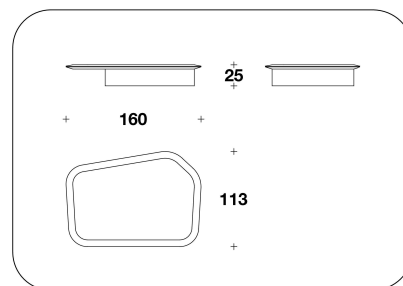
CTB (44EM) MATT VENEERED TOP+TOP INSERT : COFFEE TABLE 160x113x25H.cm 63x44 1/3x9 3/4H."
