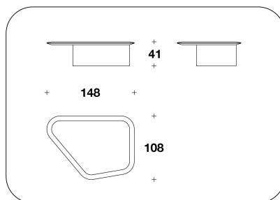
CTB (45E) GLOSSY VENEERED TOP : COFFEE TABLE 148x108x41H.cm 58 1/3x42 2/3x16 1/4H."
