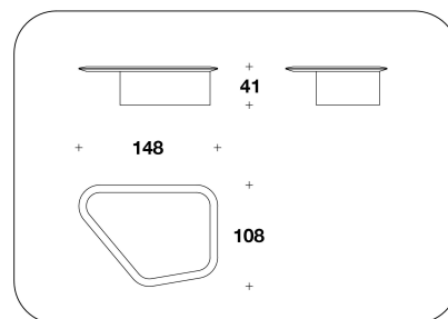
CTB (45EM) MATT VENEERED TOP+TOP INSERT : COFFEE TABLE 148x108x41H.cm 58 1/3x42 2/3x16 1/4H."
