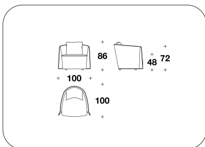
BFY (POL) POLTRONA / ARMCHAIR 100x100x86H. - H.S.45 - H.B.72cm 39 1/3x39 1/3x34H. - H.S.17 3/4 - H.B.28 1/3"
