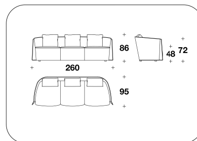
BFY (BD3) MAXI : DIVANO 3 POSTI / 3 SEATER SOFA 260x95x86H. - H.S.48 - H.B.72cm 102 1/3x37 1/3x34H. - H.S.19 - H.B.28 1/3"
